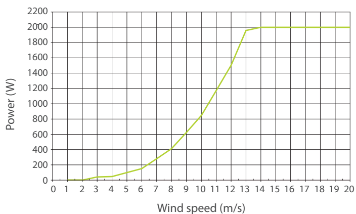
Power curve
