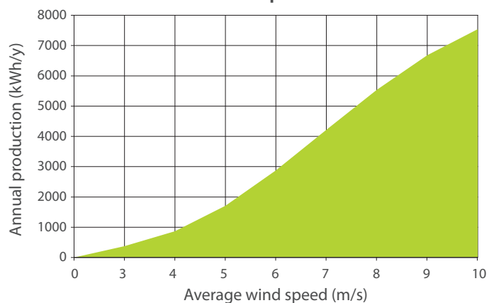
Potential production
